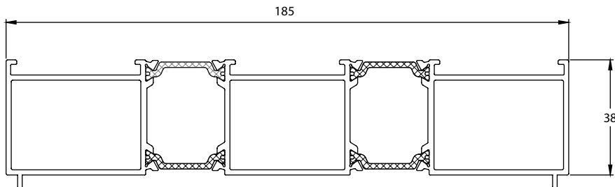
A-07141 3-TRACK 38mm FRAME EXTENDER
